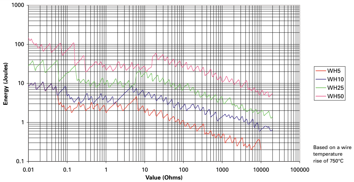
WH Series "Energy Capability" Graph
