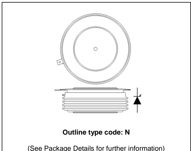
Fig. 1 Package outline
