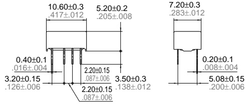
External dimensions
