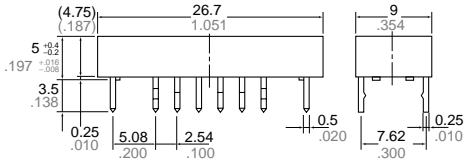
Self-clinching terminal
