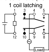
Pin layout and schematic (BOTTOM VIEW)
