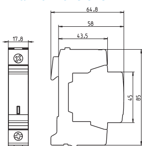
OVR T2 40-275 P OVR T2 40-275s P OVR T2 70-275s P OVR T2 70 N P
